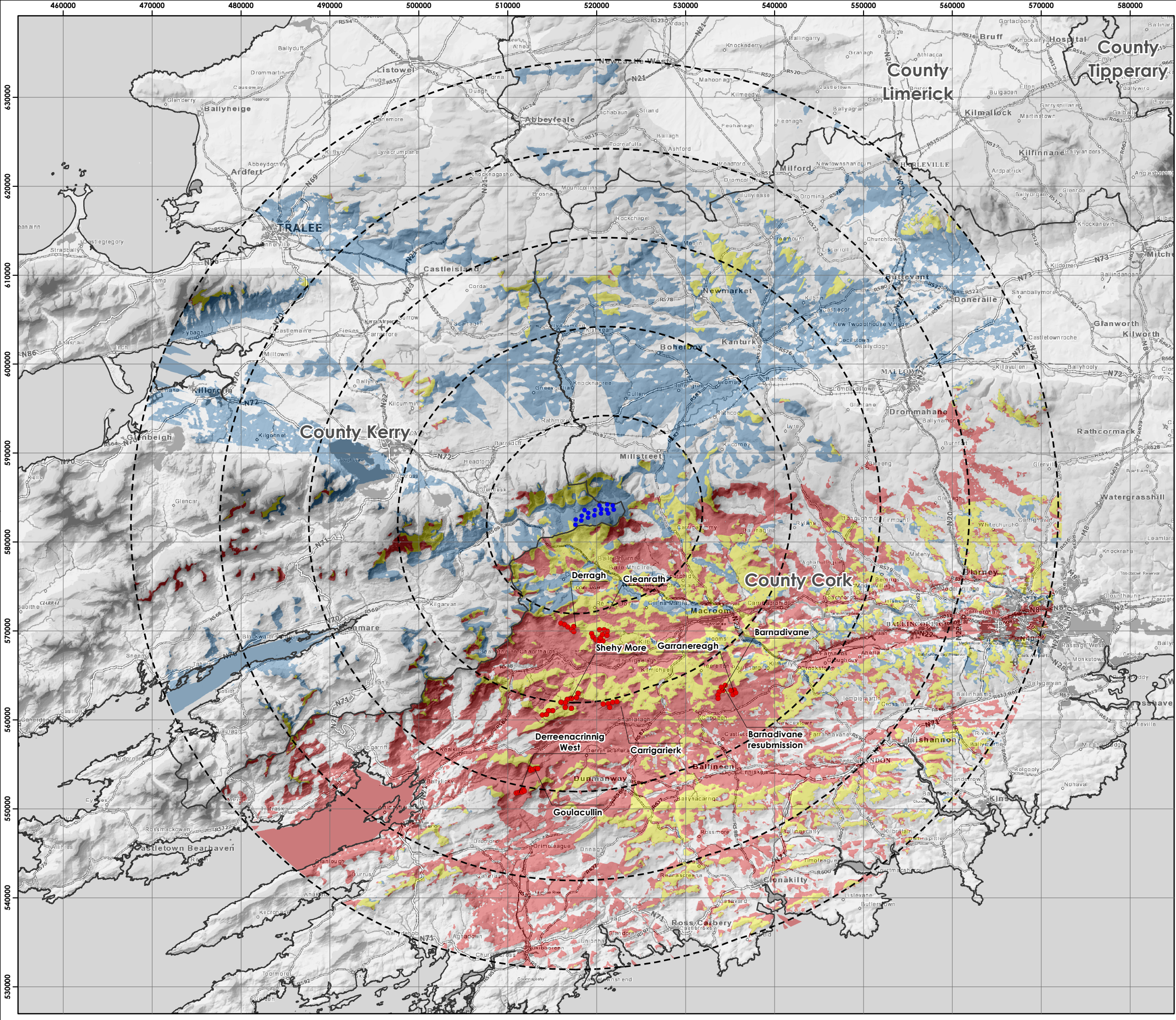
Figure 6-11 South Wind Farm Group Comparative ZTV (Operational and Consented)
